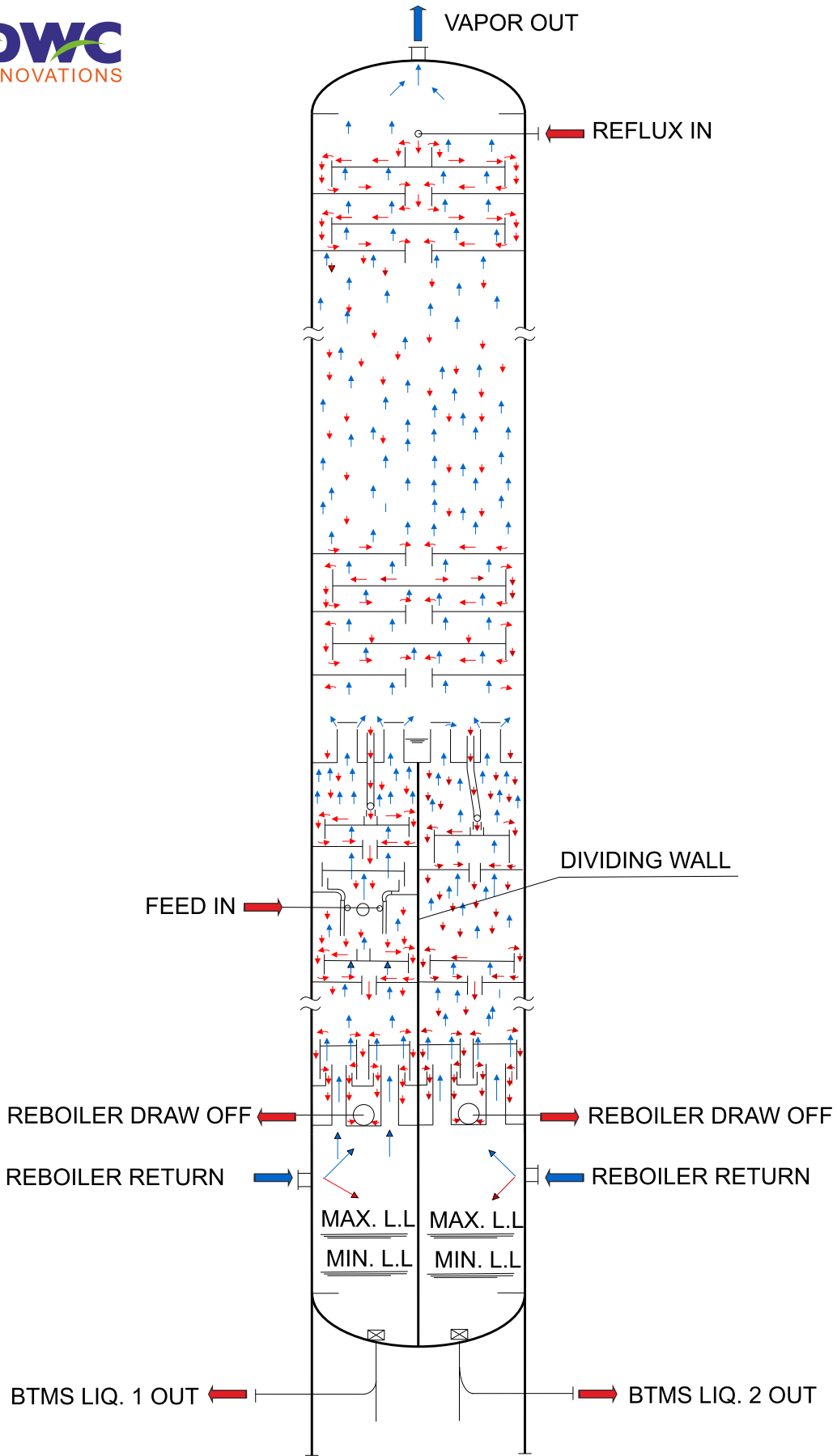
BOTTOM DIVIDING WALL COLUMN
