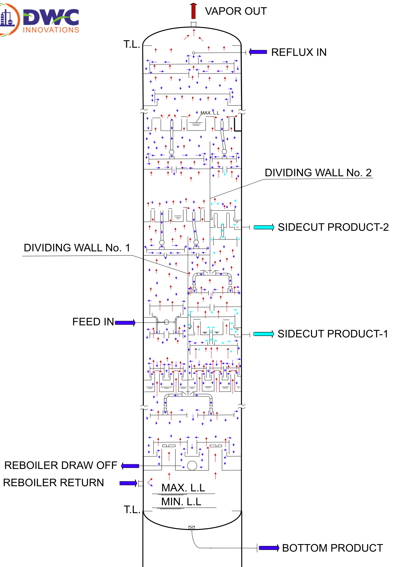
DUAL DIVIDING WALL COLUMN
