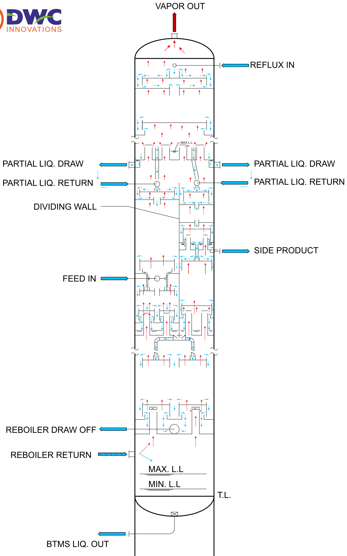
MIDDLE DIVIDING WALL COLUMN
