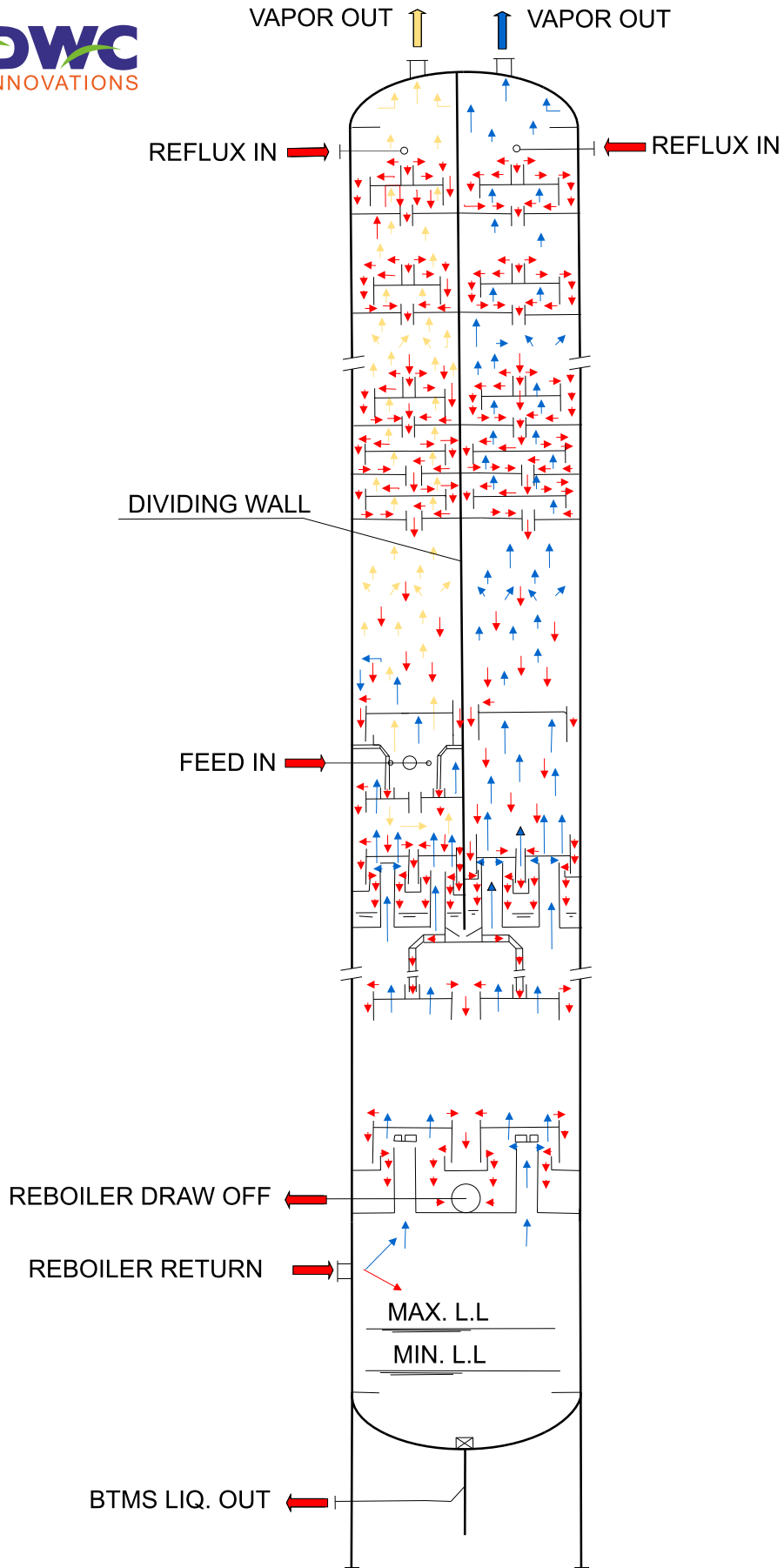
TOP DIVIDING WALL COLUMN
